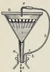
FIG. 26.—Varnish Filter.
